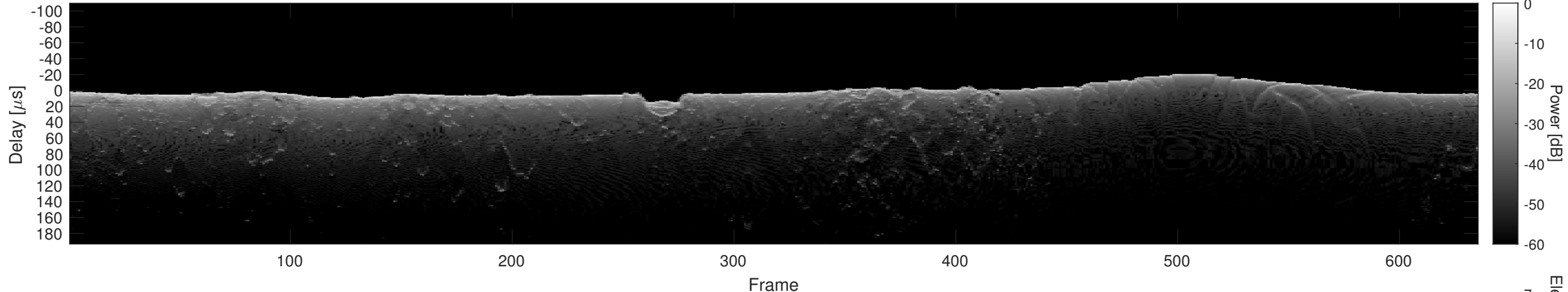
Orbit 4536, Cluttergram
