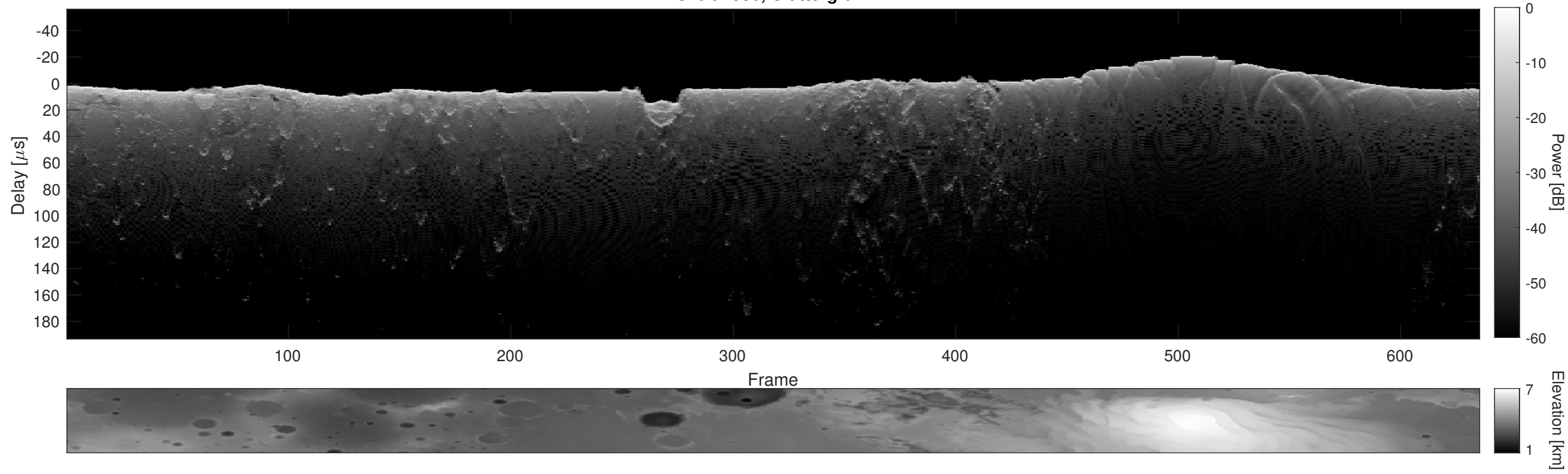
Orbit 4536, Cluttergram
