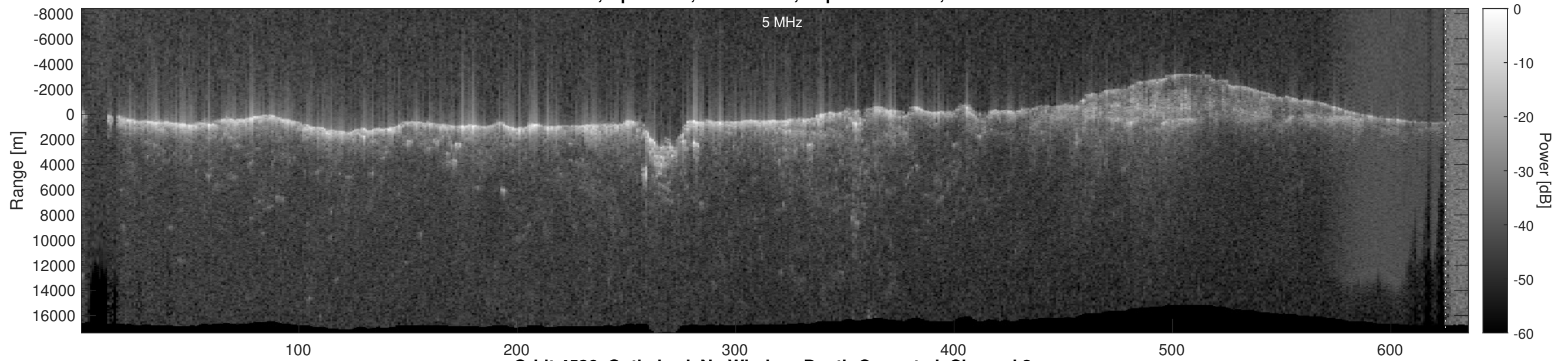
Orbit 4536, Optimized, No Window, Depth-Corrected, Channel 2
