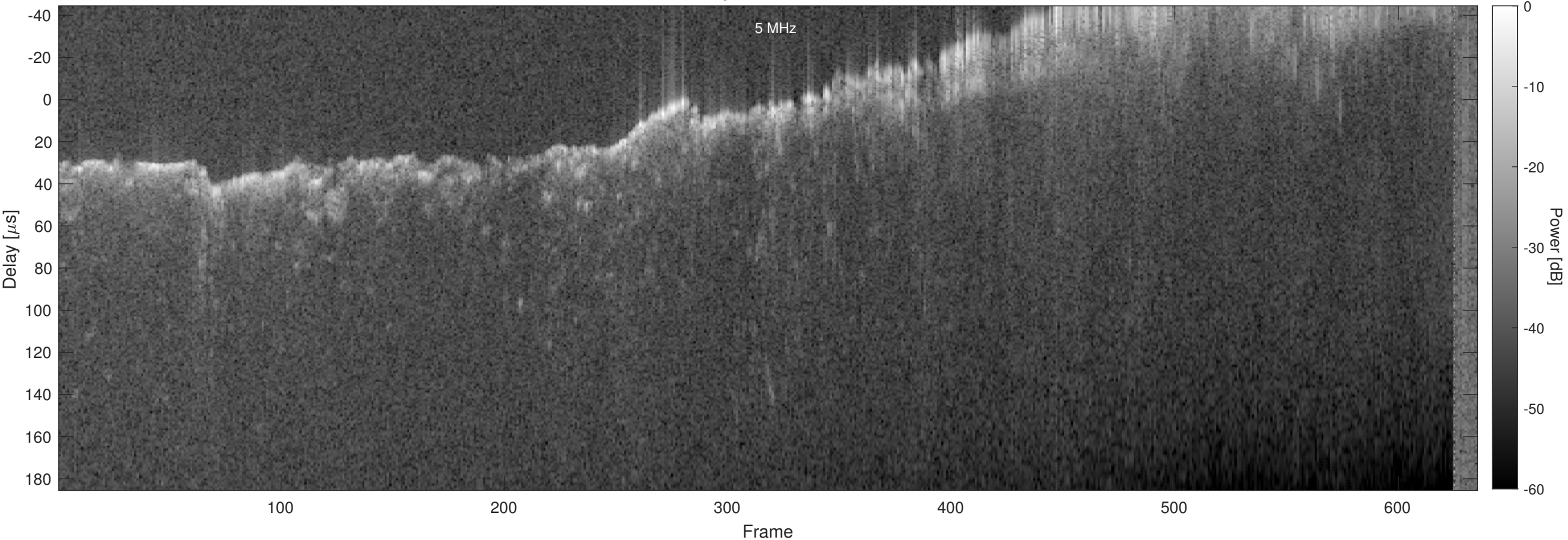
Orbit 4537, Chapman, Window, Channel 2
