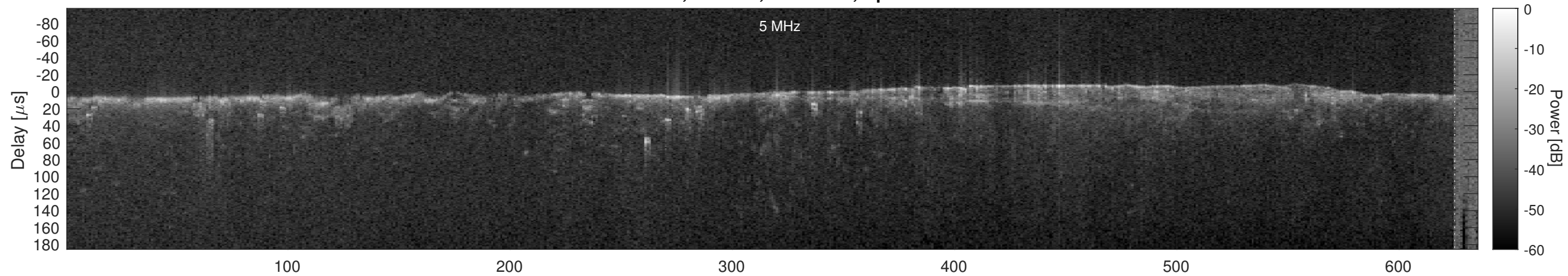
Orbit 4537, Cluttergram
