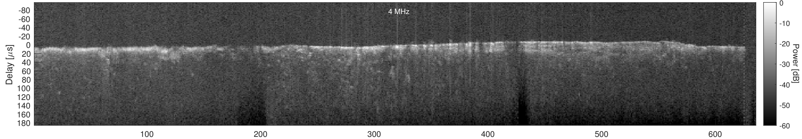
Orbit 4537, Cluttergram
