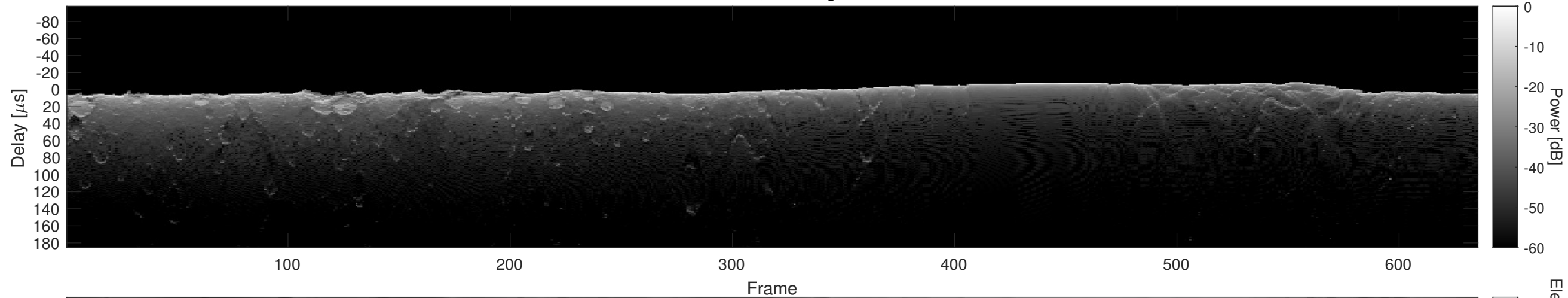
Orbit 4537, Cluttergram
