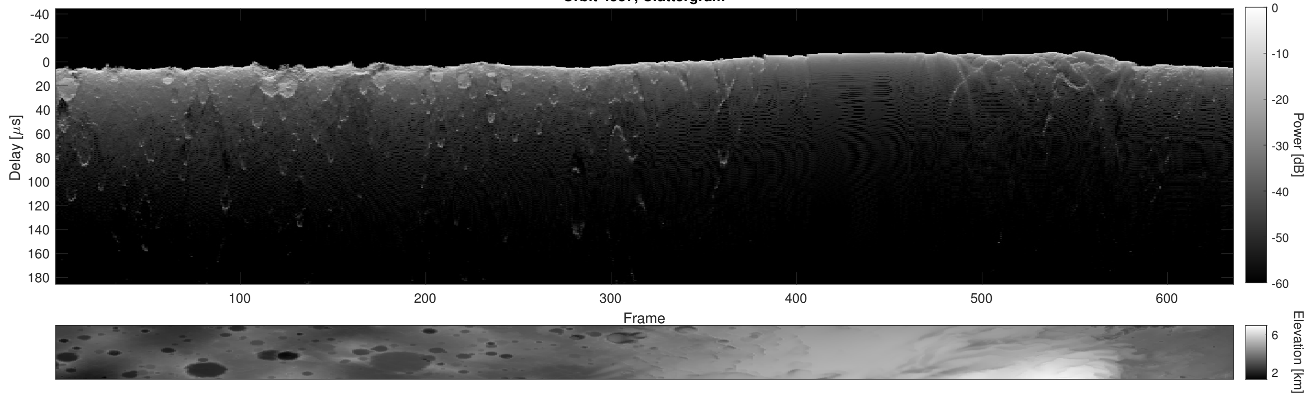
Orbit 4537, Cluttergram
