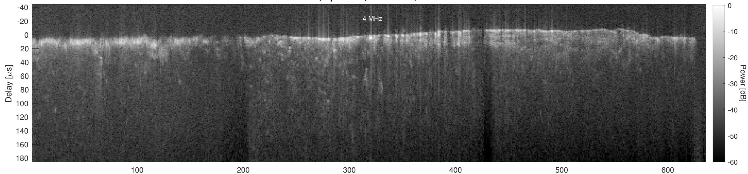
Orbit 4537, Cluttergram
