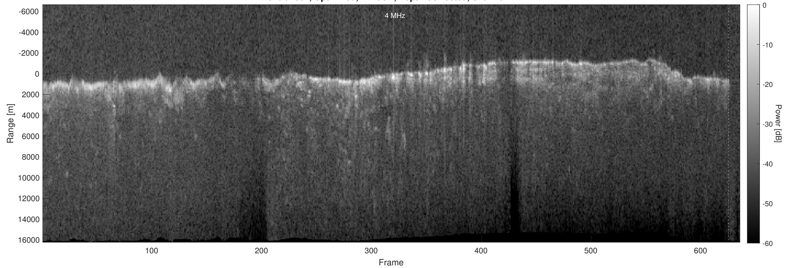
Orbit 4537, Optimized, Window, Depth-Corrected, Channel 2
