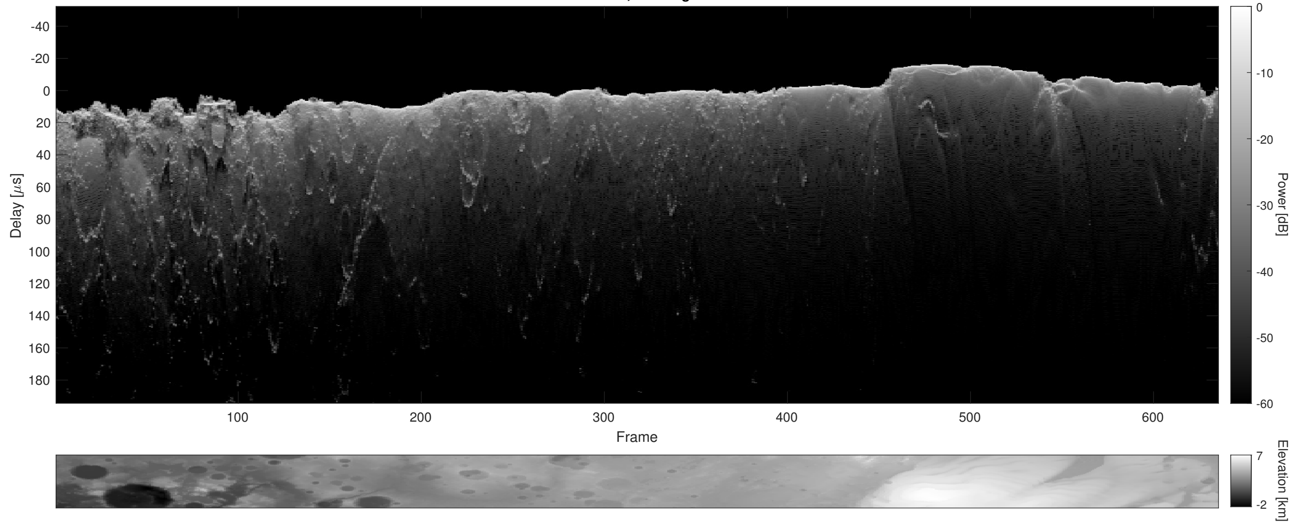
Orbit 4539, Cluttergram
