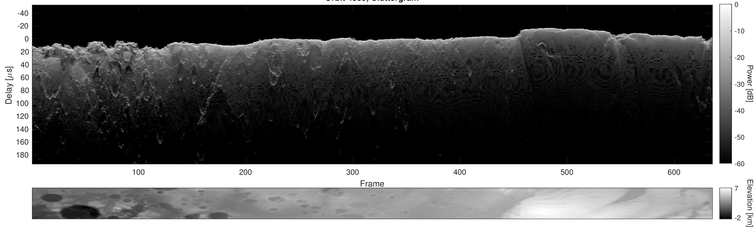
Orbit 4539, Cluttergram
