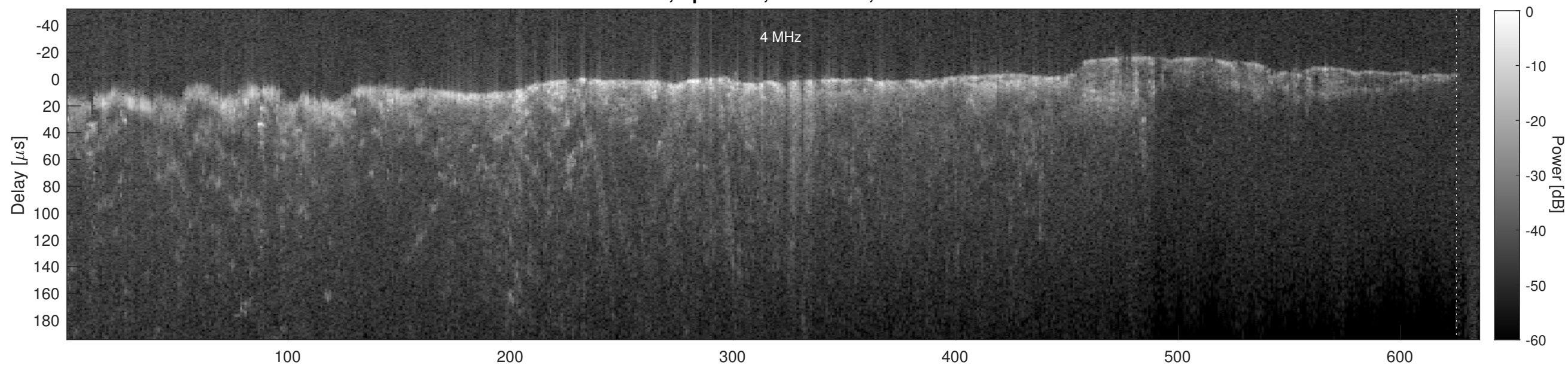
Orbit 4539, Cluttergram
