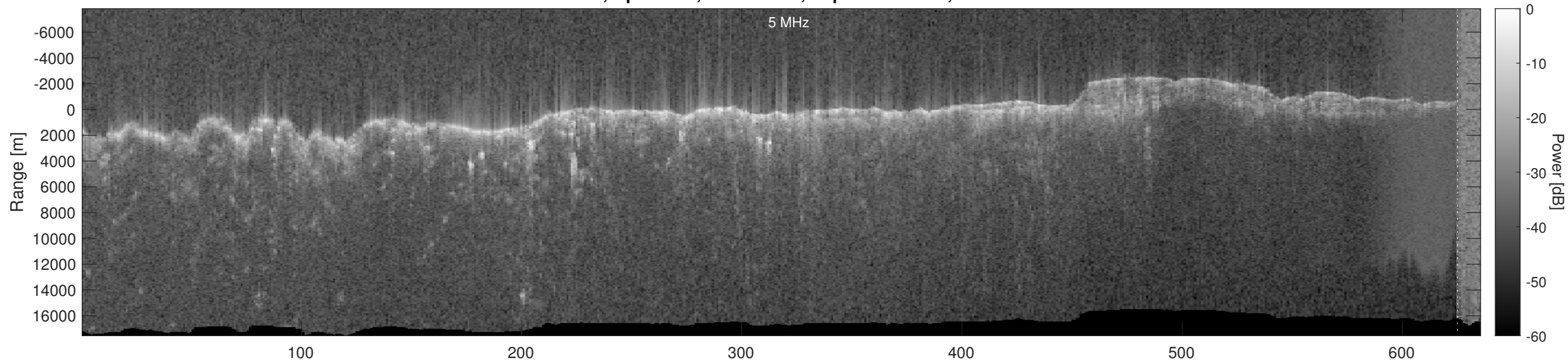
Orbit 4539, Optimized, No Window, Depth-Corrected, Channel 2
