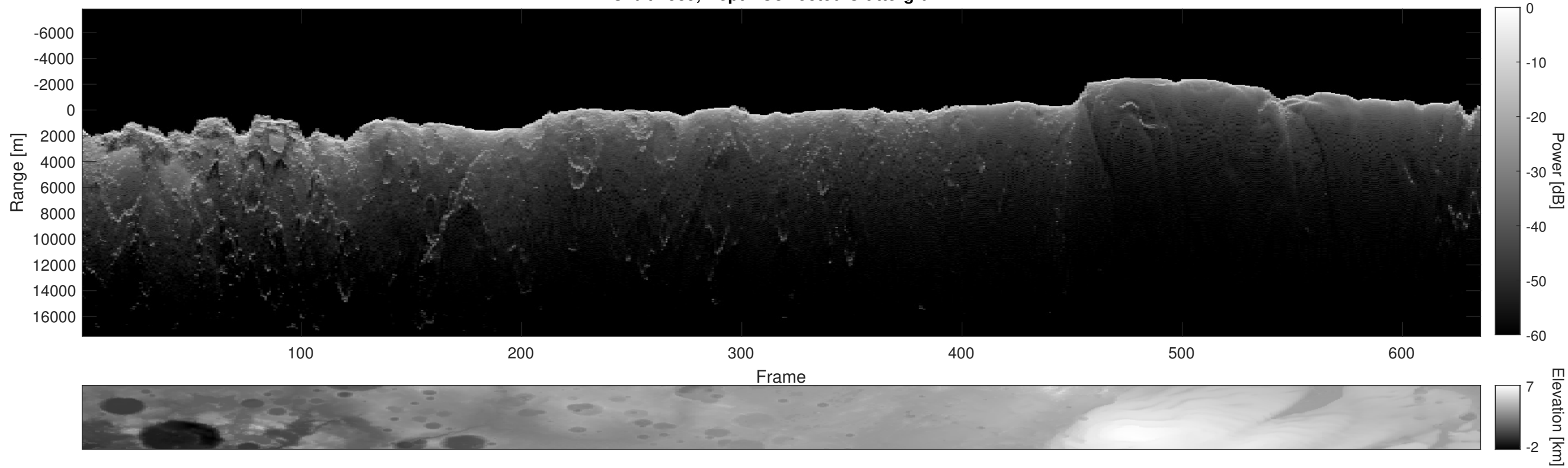
Orbit 4539, Depth-Corrected Cluttergram
