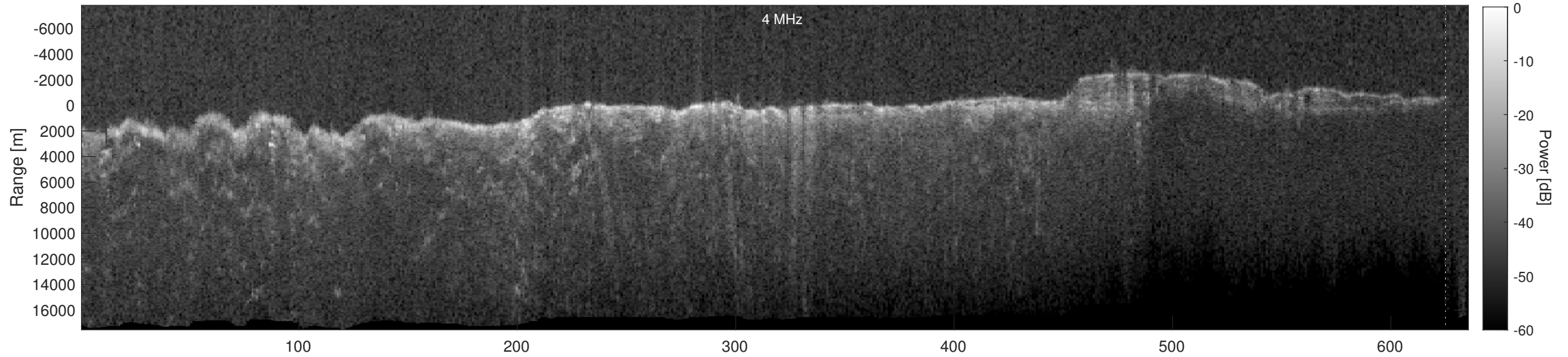
Orbit 4539, Depth-Corrected Cluttergram
