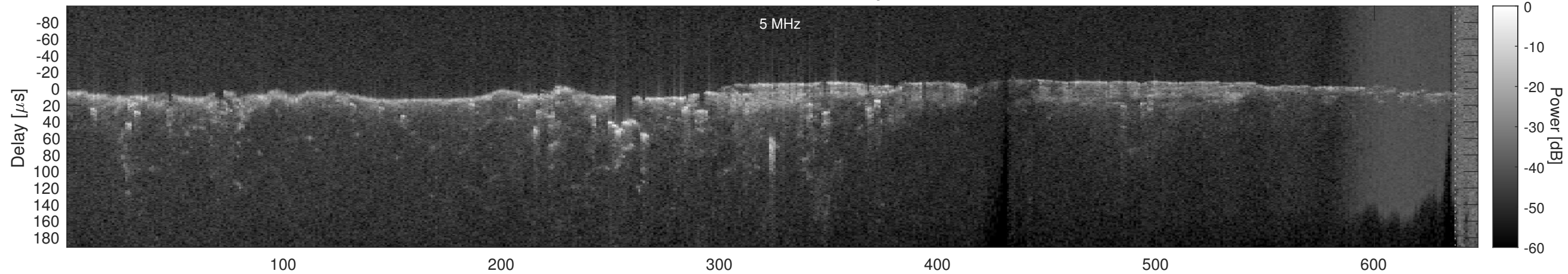
Orbit 4541, Cluttergram
