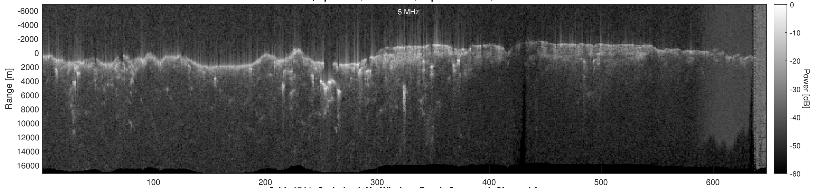
Orbit 4541, Optimized, No Window, Depth-Corrected, Channel 2
