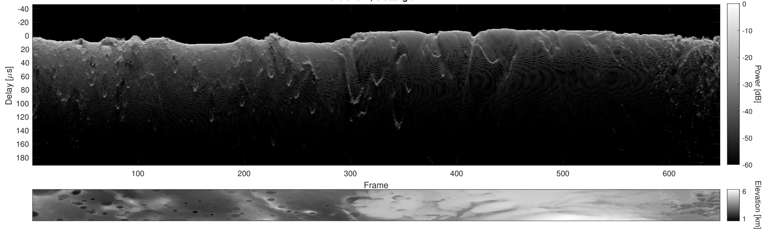
Orbit 4541, Cluttergram
