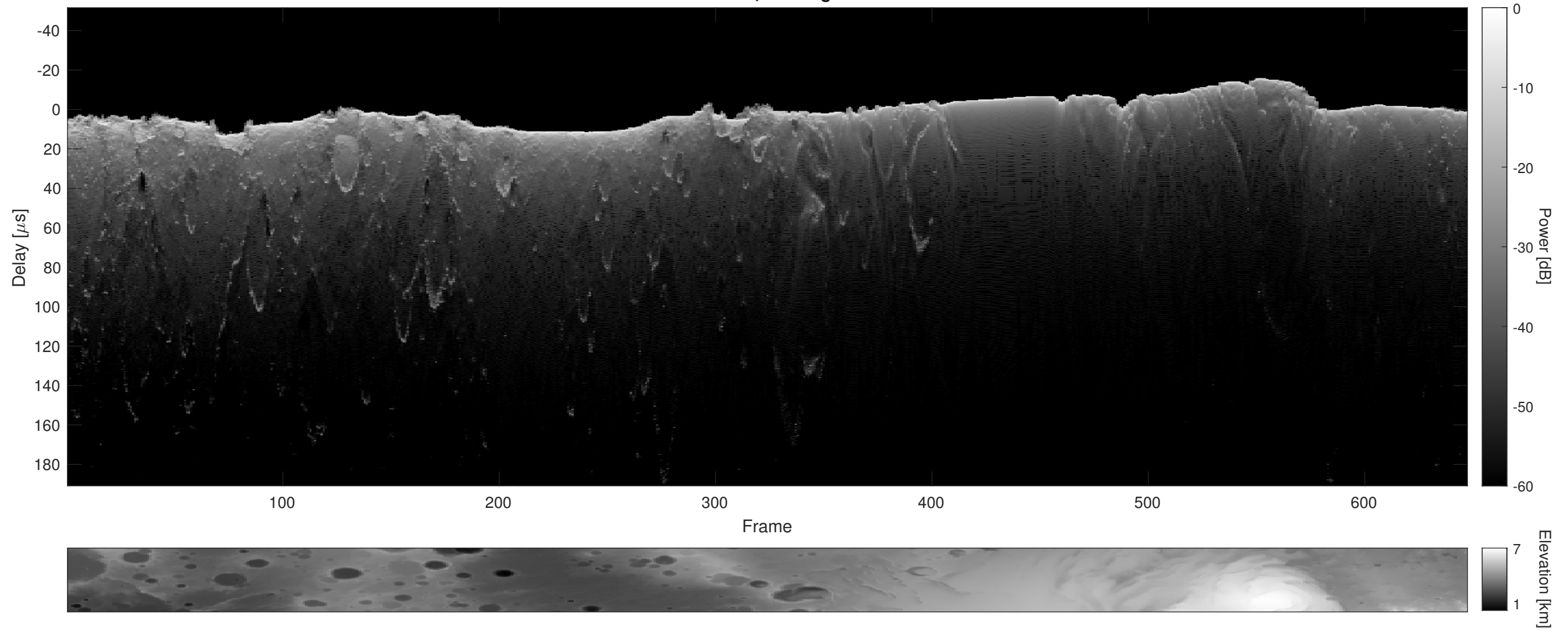
Orbit 4544, Cluttergram
