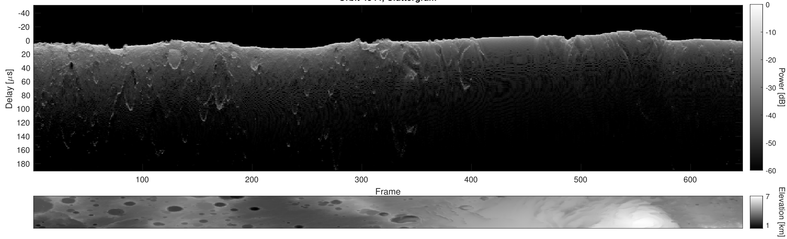
Orbit 4544, Cluttergram
