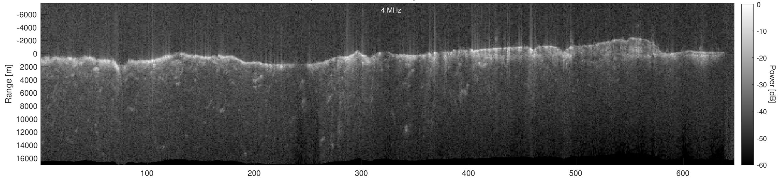
Orbit 4544, Depth-Corrected Cluttergram
