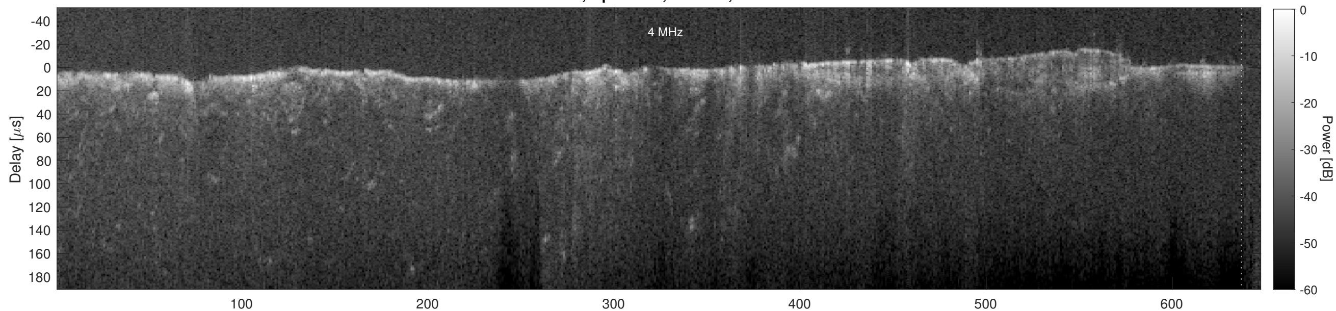
Orbit 4544, Cluttergram
