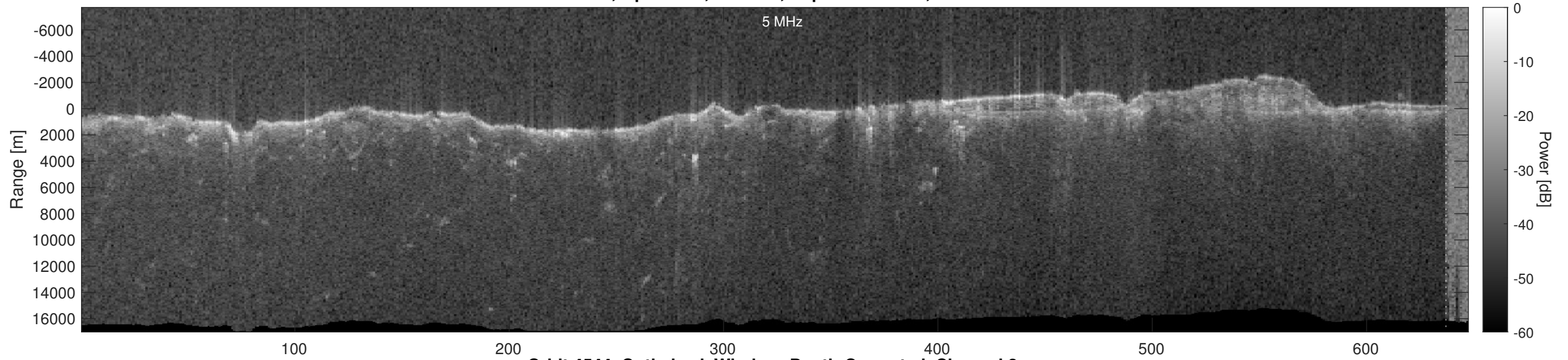
Orbit 4544, Optimized, Window, Depth-Corrected, Channel 2
