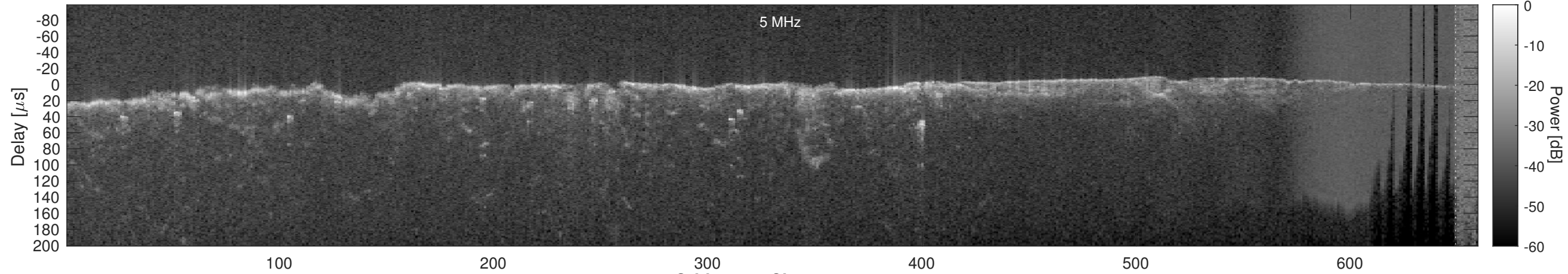
Orbit 4545, Cluttergram
