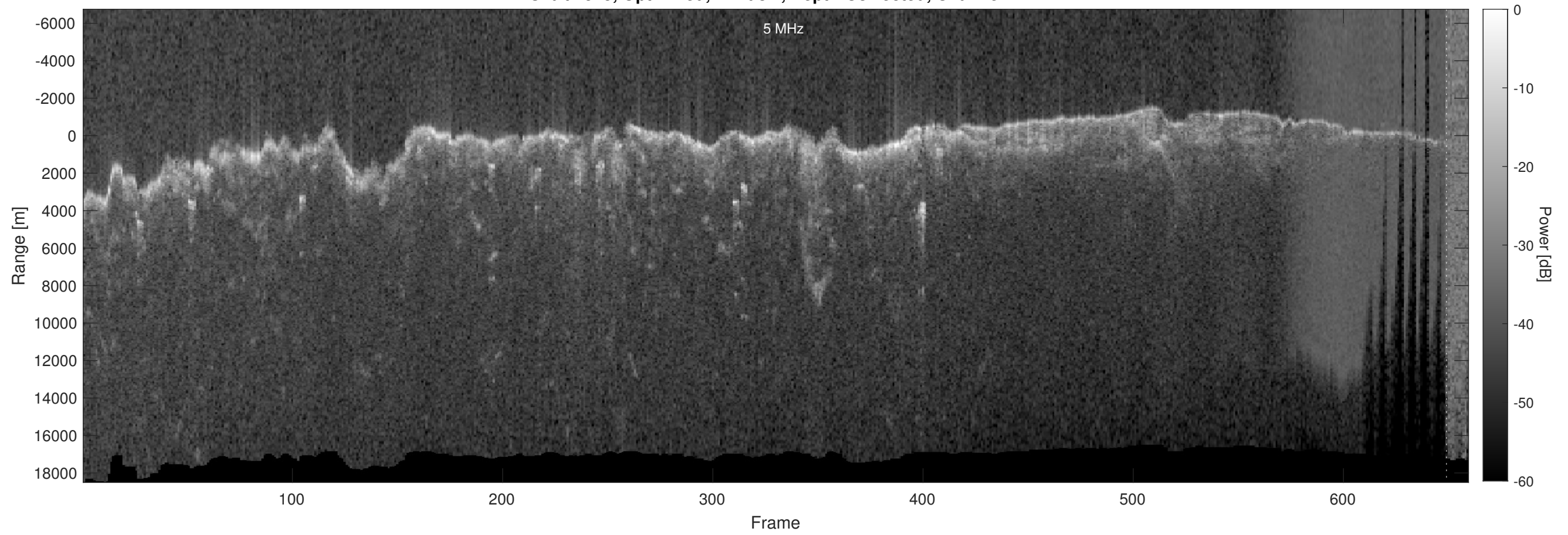
Orbit 4545, Optimized, Window, Depth-Corrected, Channel 2
