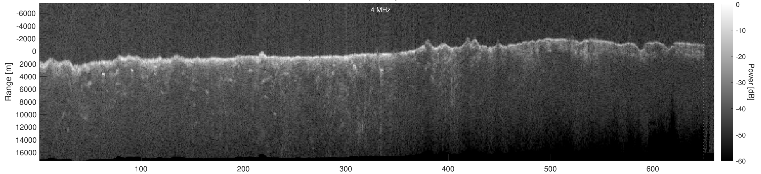
Orbit 4546, Depth-Corrected Cluttergram
