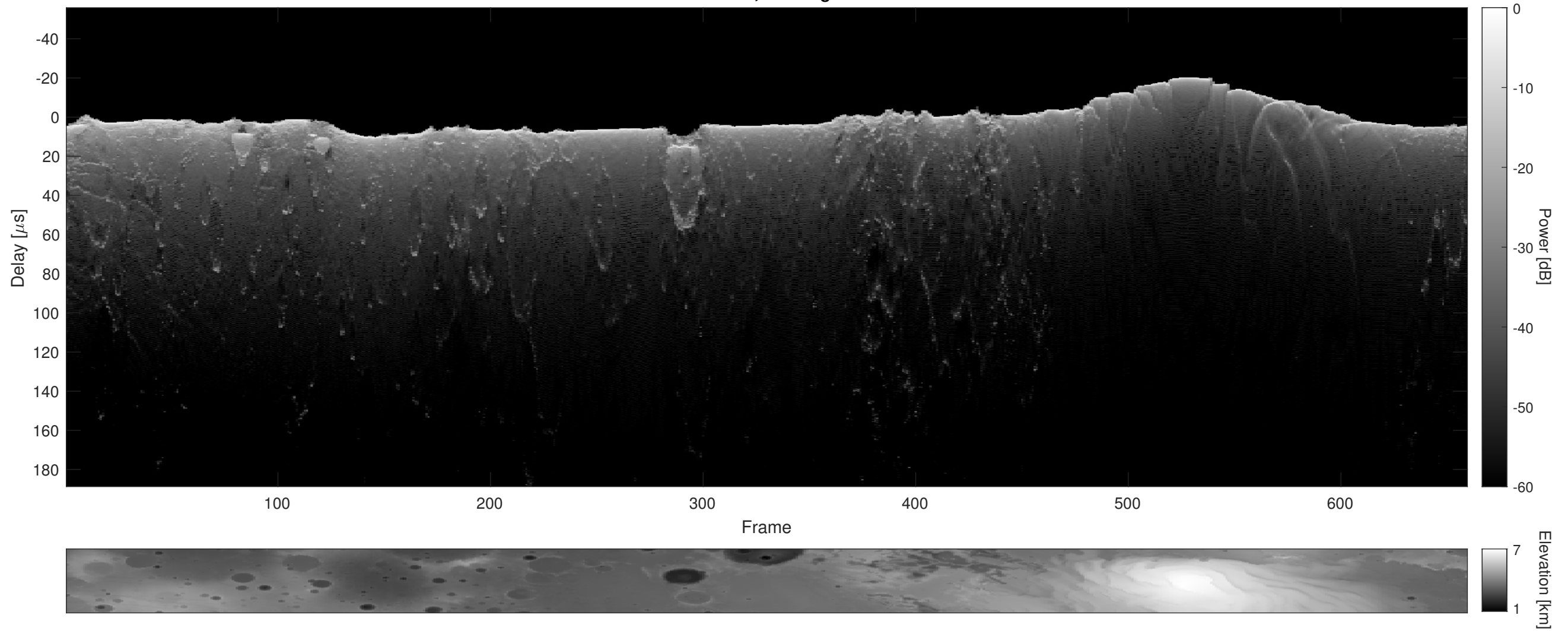
Orbit 4547, Cluttergram
