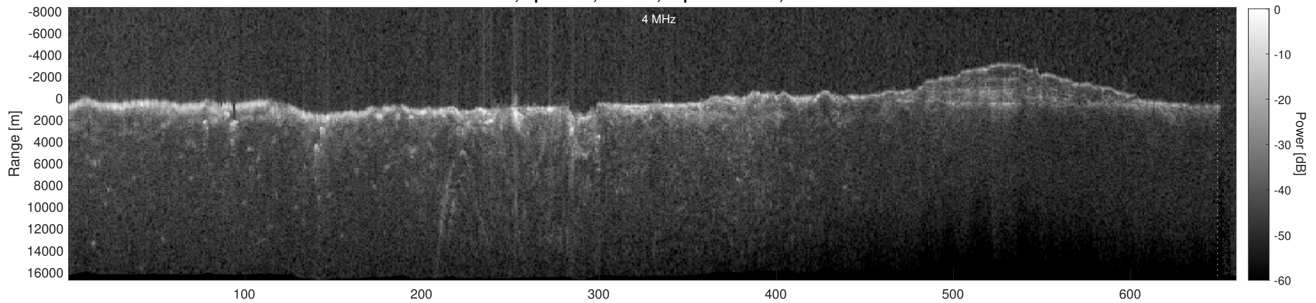
Orbit 4547, Depth-Corrected Cluttergram
