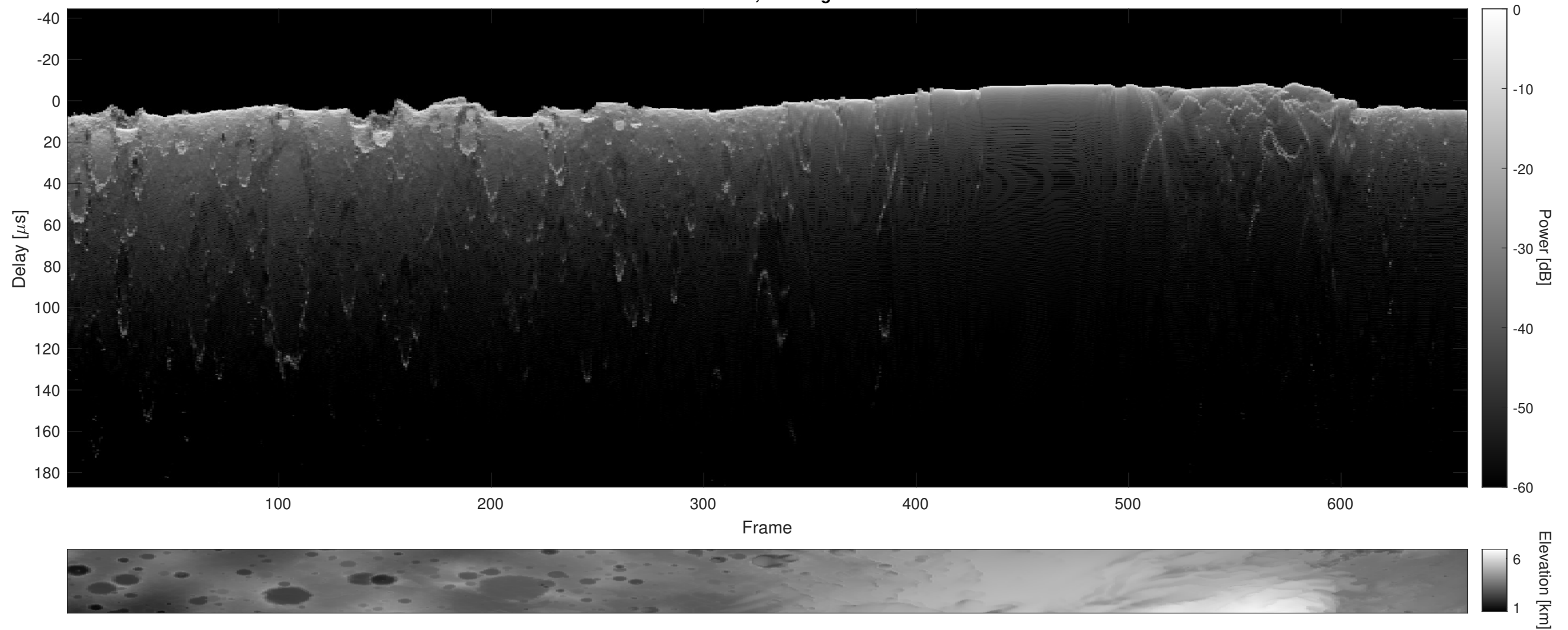
Orbit 4548, Cluttergram
