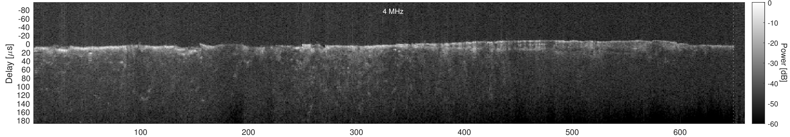
Orbit 4548, Cluttergram
