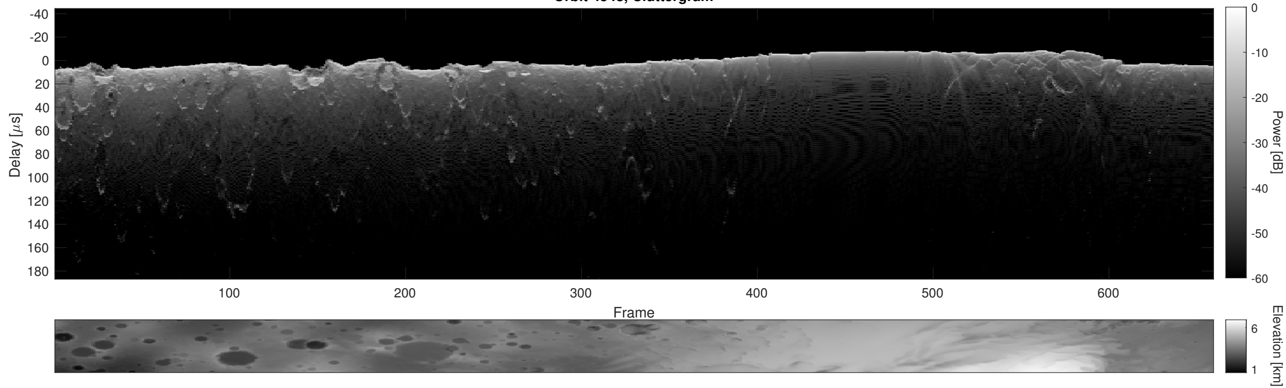
Orbit 4548, Cluttergram
