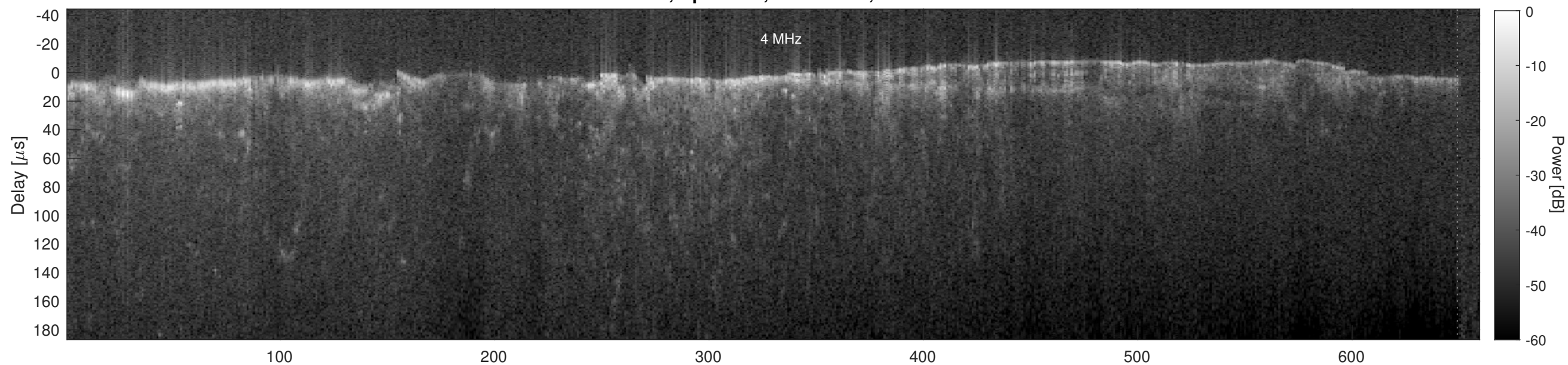
Orbit 4548, Cluttergram
