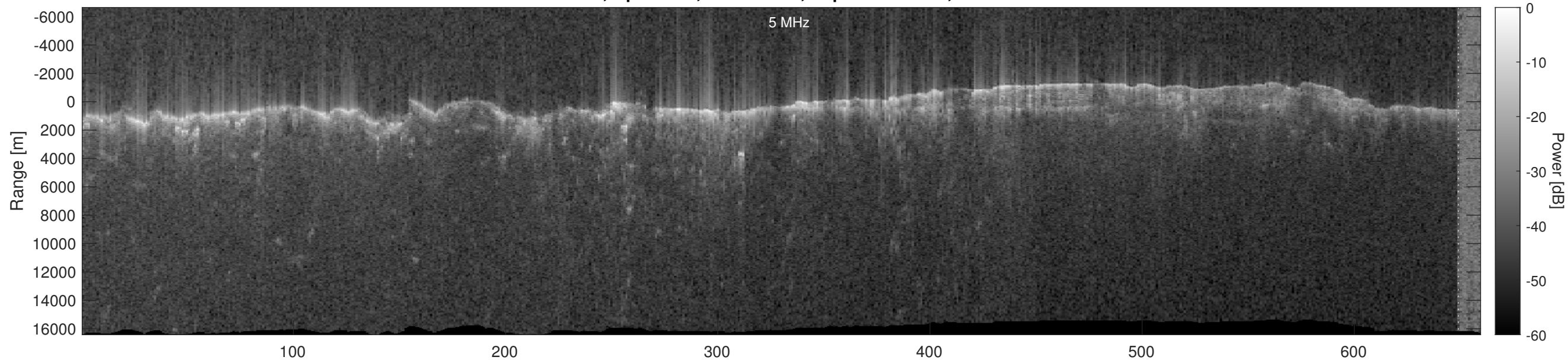
Orbit 4548, Optimized, No Window, Depth-Corrected, Channel 2
