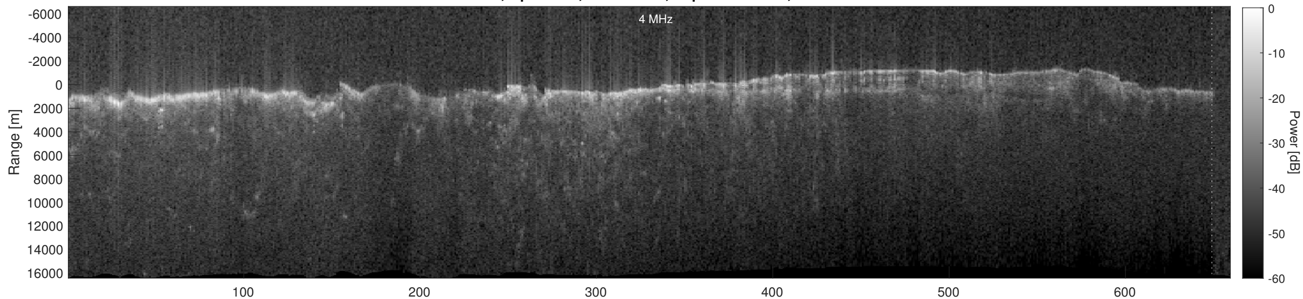
Orbit 4548, Depth-Corrected Cluttergram
