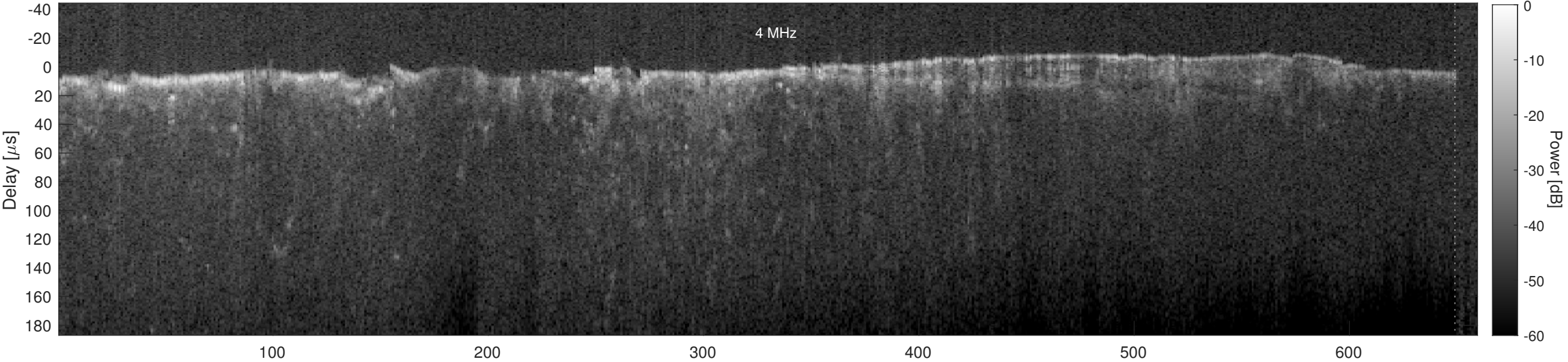
Orbit 4548, Cluttergram
