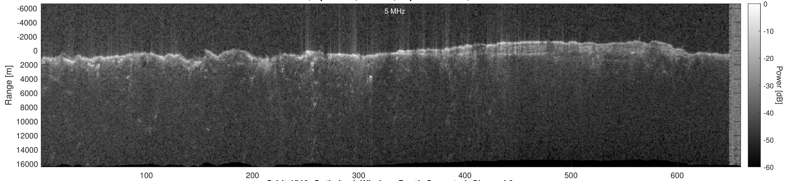
Orbit 4548, Optimized, Window, Depth-Corrected, Channel 2
