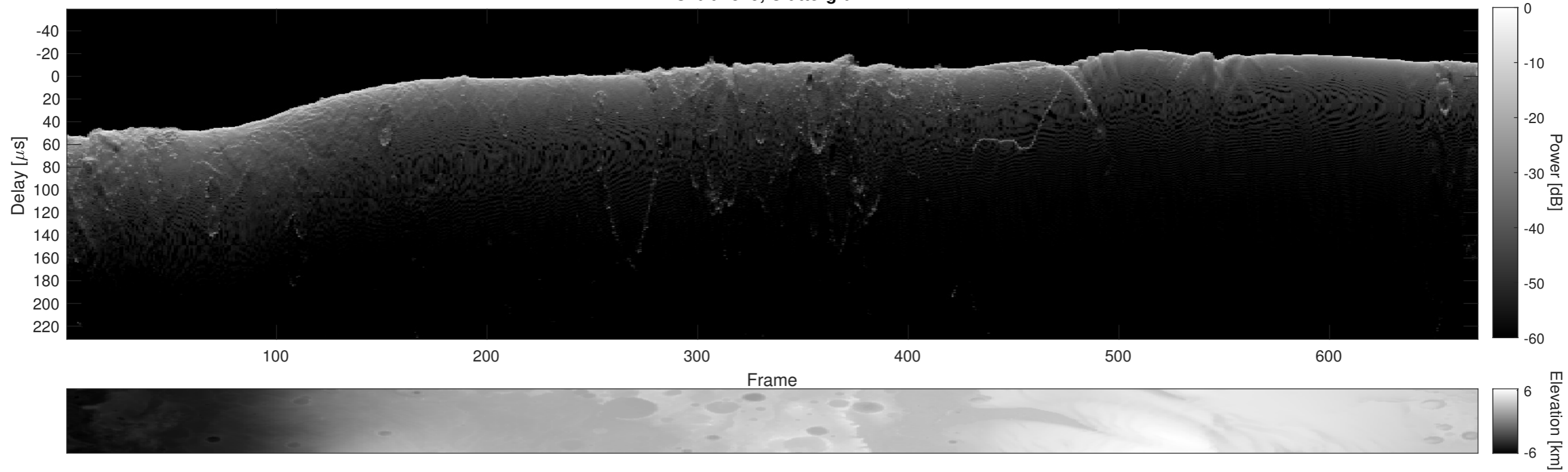
Orbit 4549, Cluttergram
