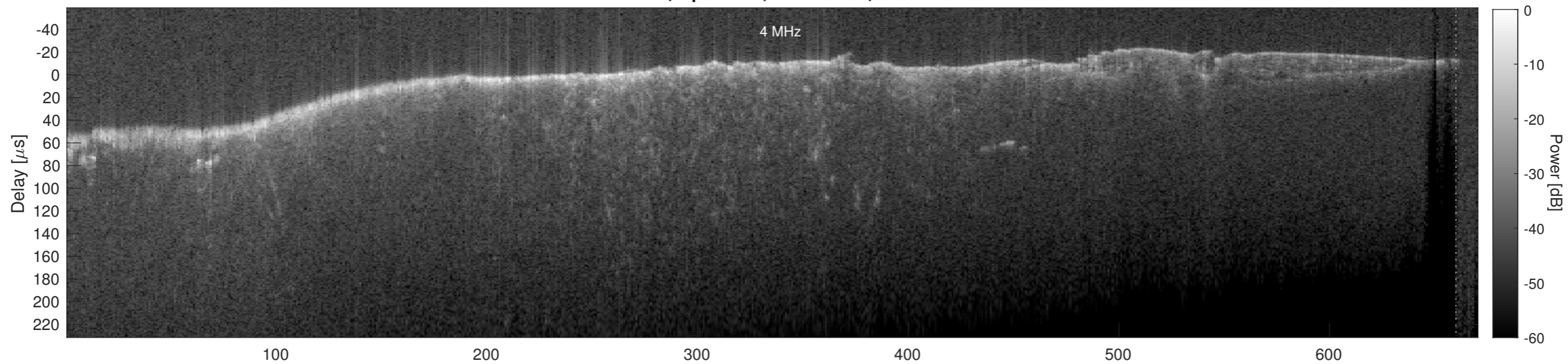
Orbit 4549, Cluttergram
