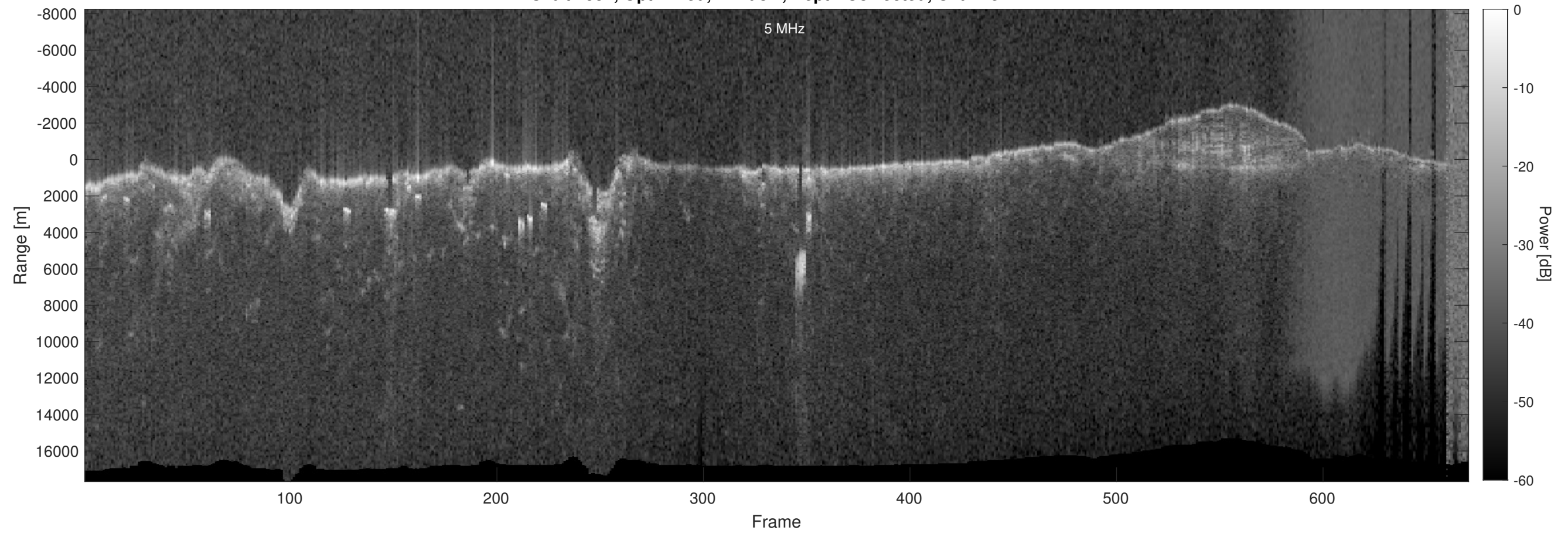
Orbit 4551, Optimized, Window, Depth-Corrected, Channel 2
