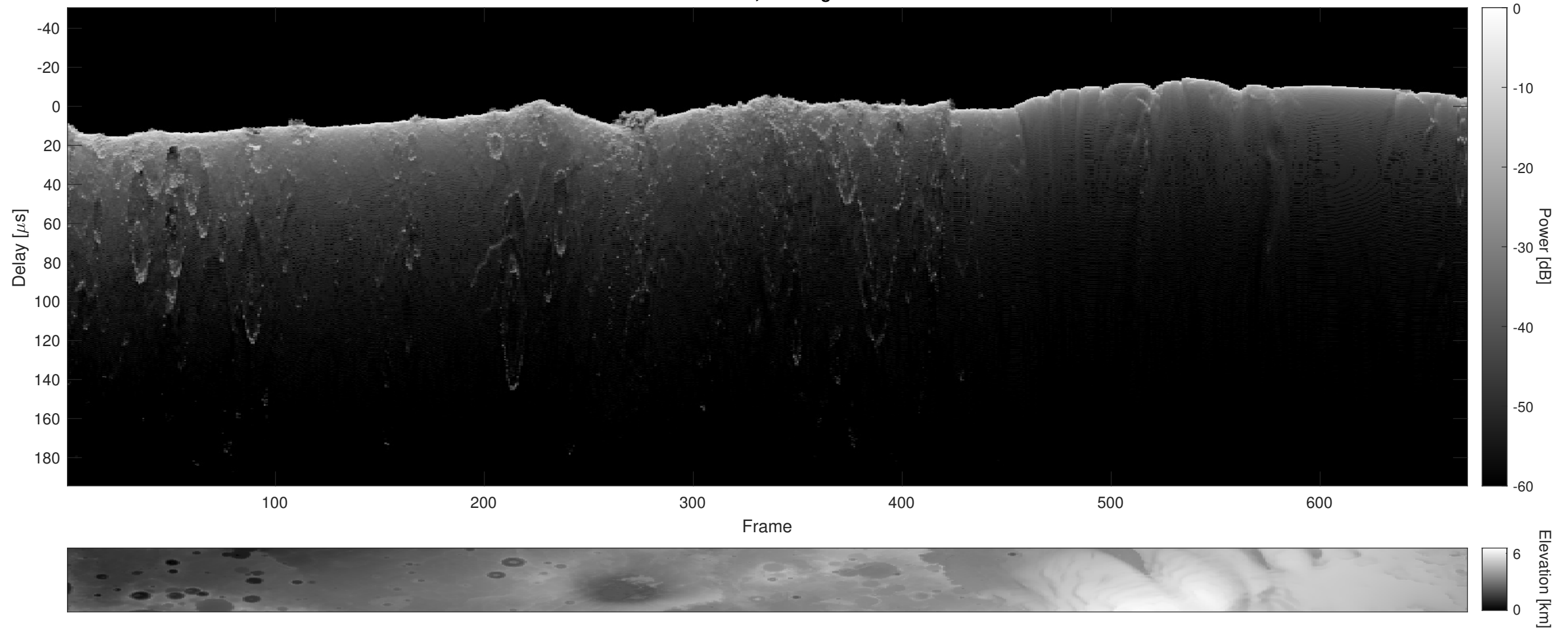
Orbit 4553, Cluttergram
