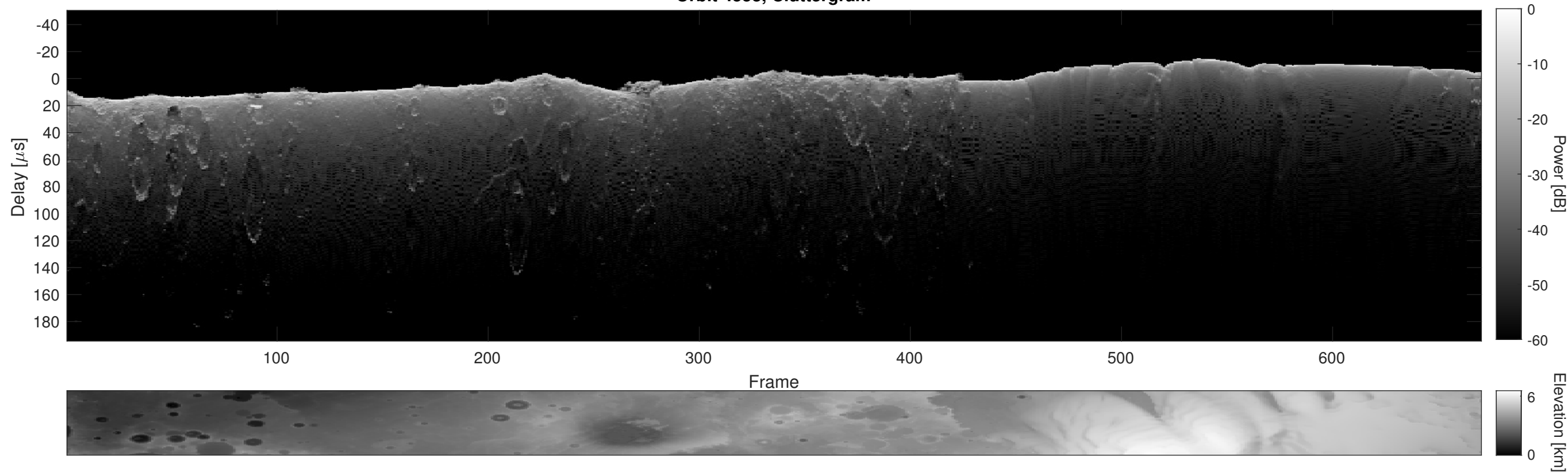
Orbit 4553, Cluttergram
