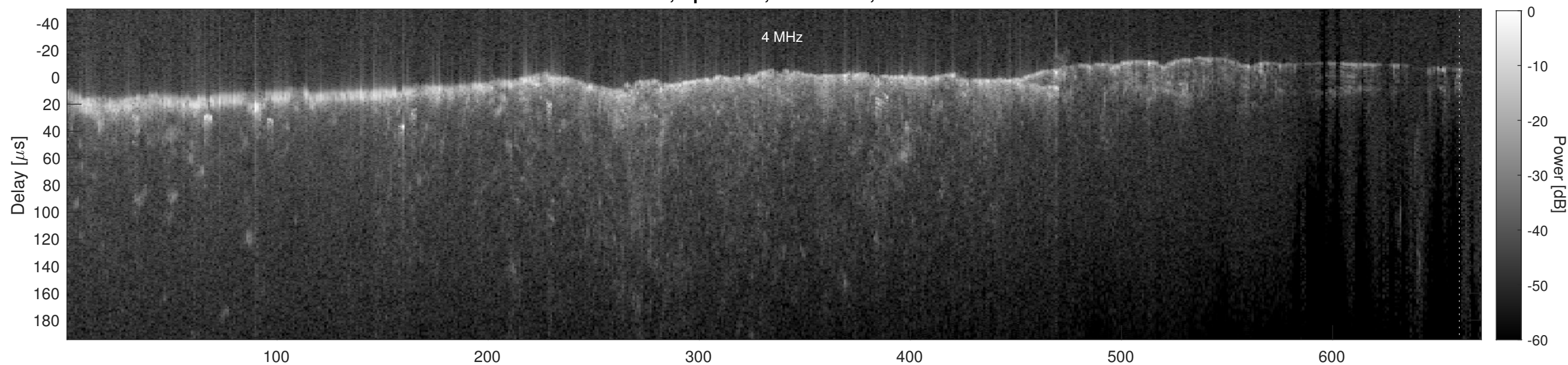
Orbit 4553, Cluttergram
