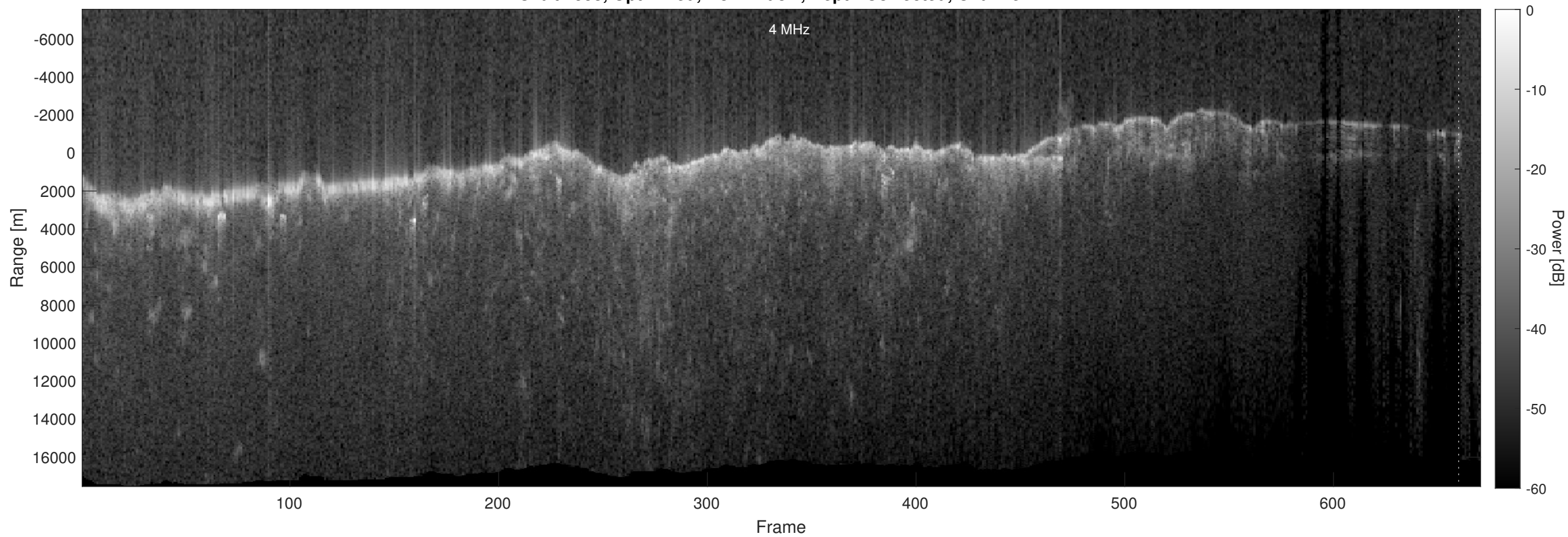
Orbit 4553, Optimized, No Window, Depth-Corrected, Channel 2
