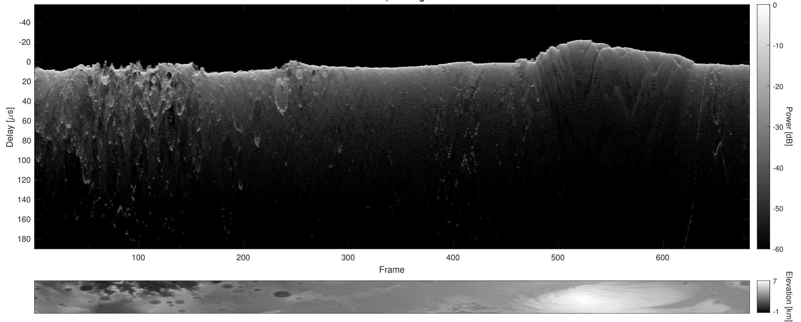
Orbit 4554, Cluttergram
