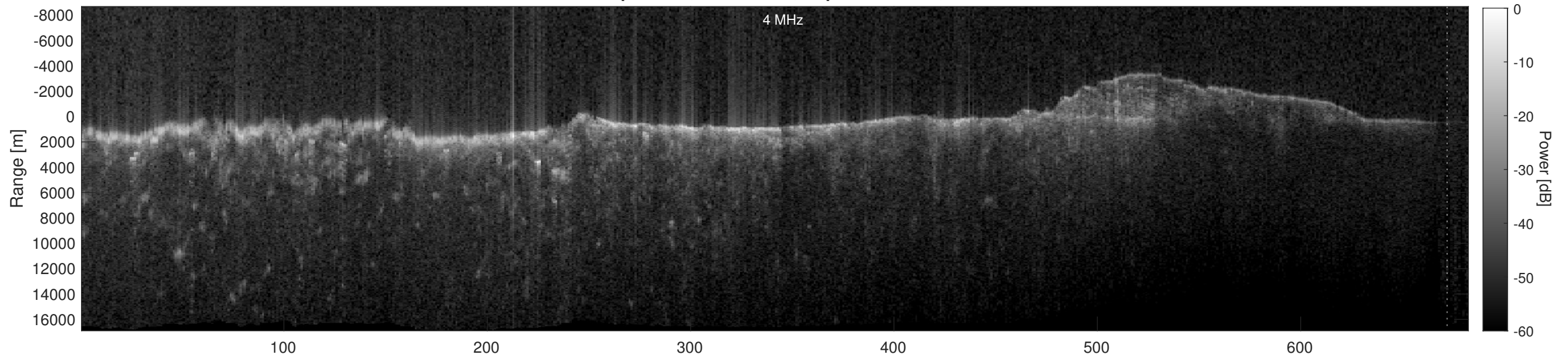
Orbit 4554, Depth-Corrected Cluttergram
