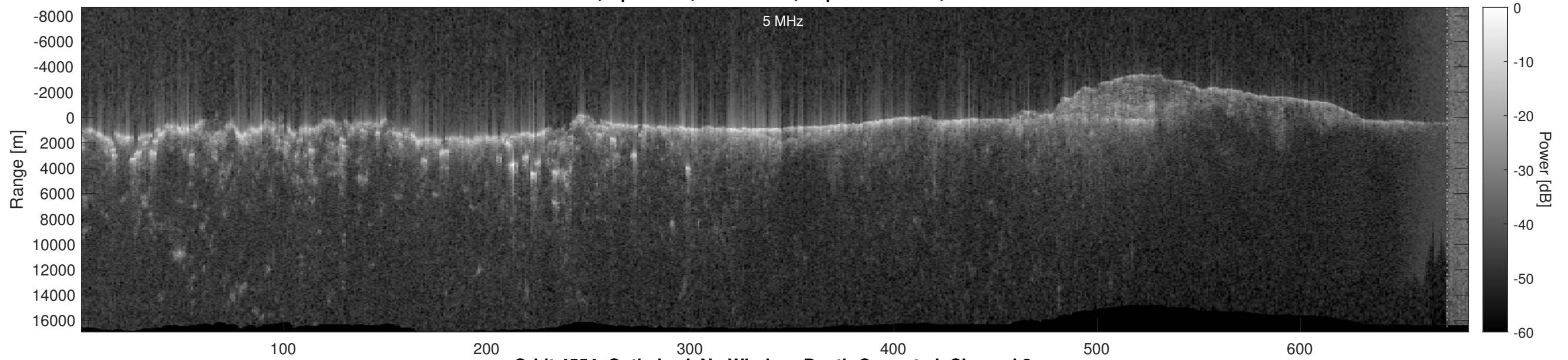
Orbit 4554, Optimized, No Window, Depth-Corrected, Channel 2
