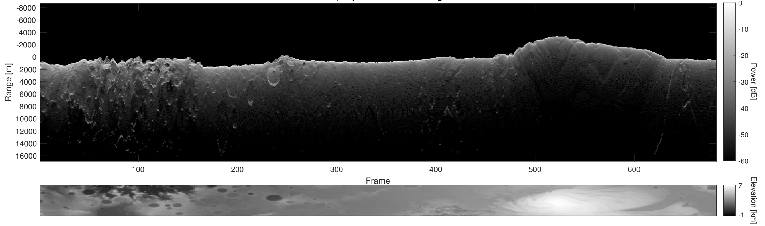
Orbit 4554, Depth-Corrected Cluttergram
