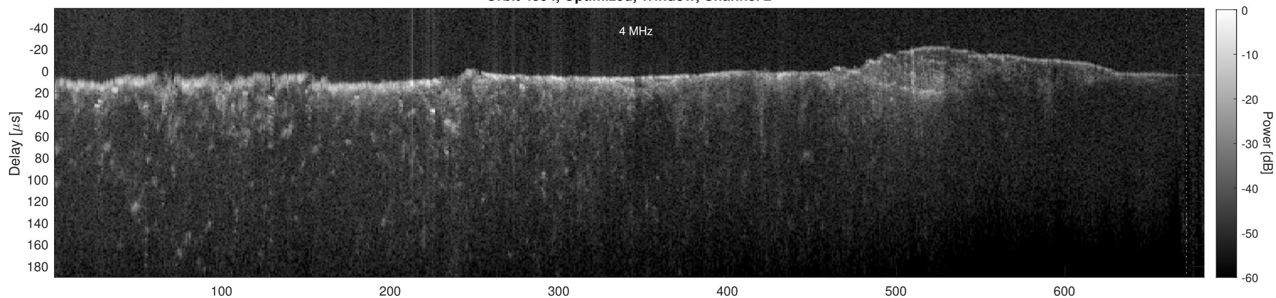
Orbit 4554, Cluttergram
