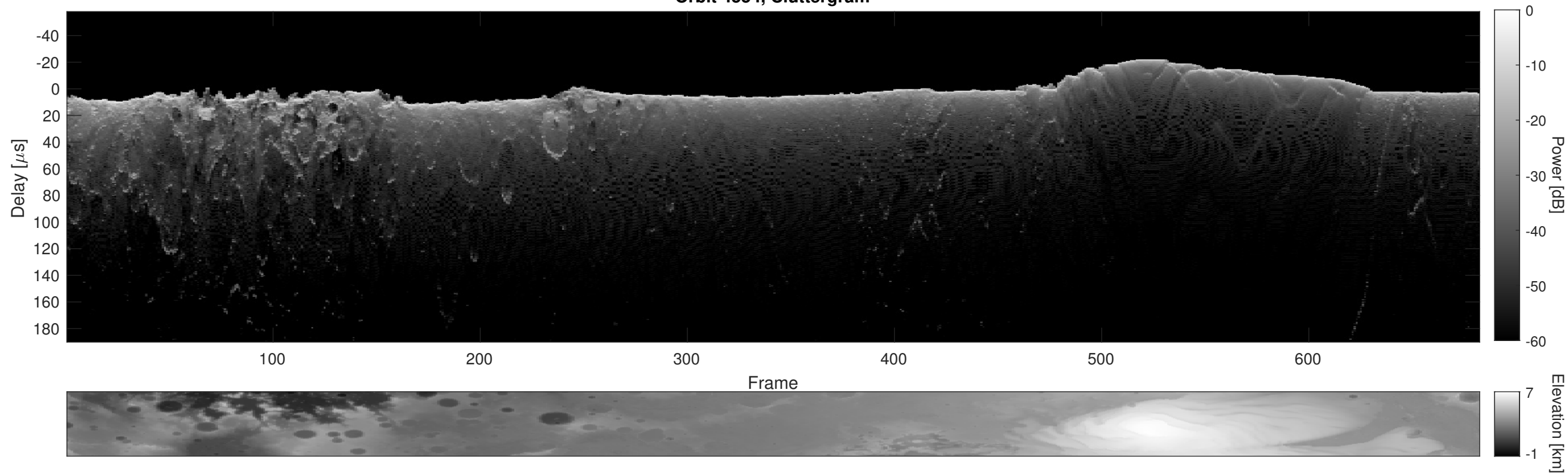
Orbit 4554, Cluttergram
