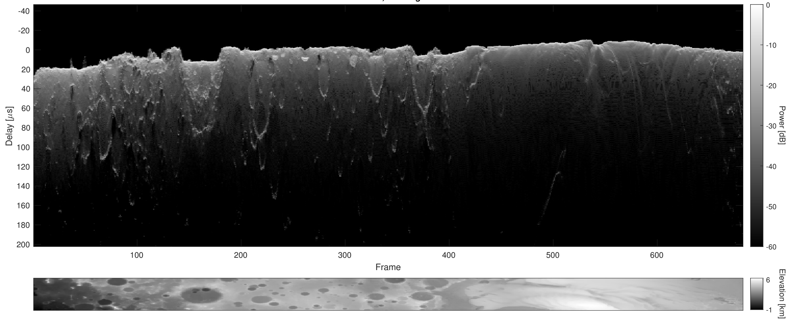
Orbit 4556, Cluttergram
