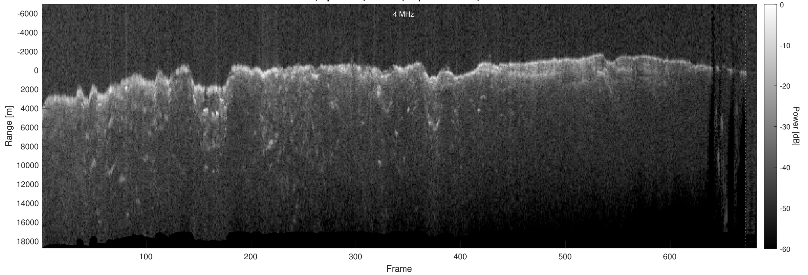
Orbit 4556, Optimized, Window, Depth-Corrected, Channel 2
