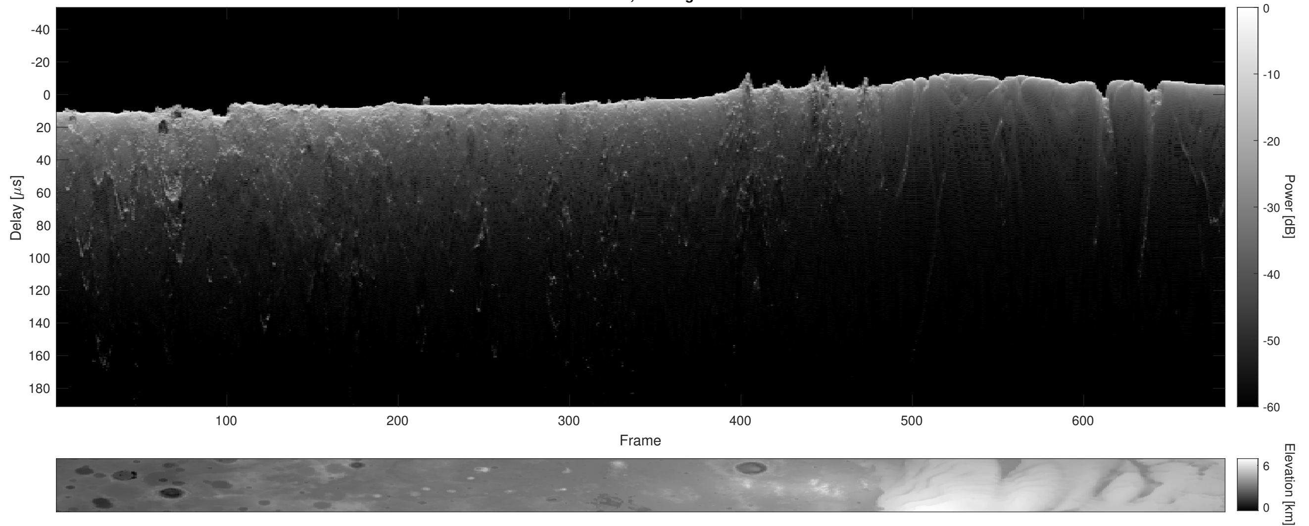
Orbit 4557, Cluttergram
