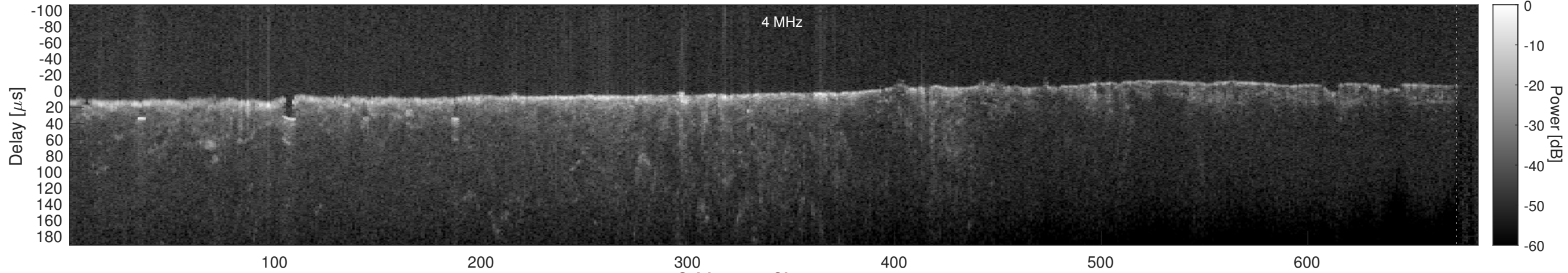
Orbit 4557, Cluttergram
