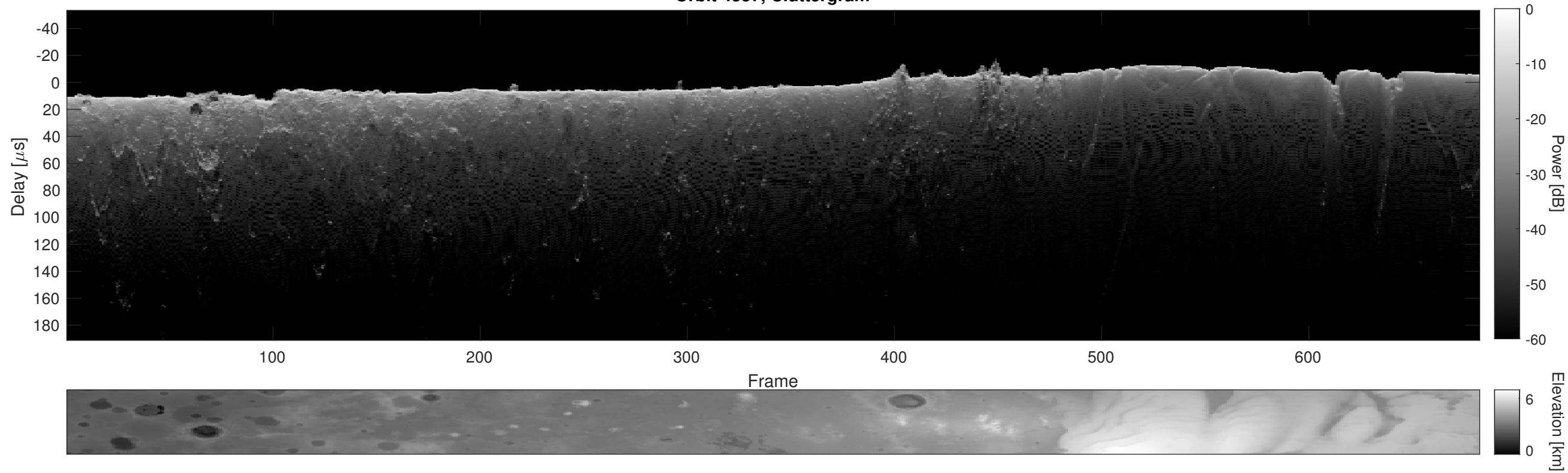
Orbit 4557, Cluttergram
