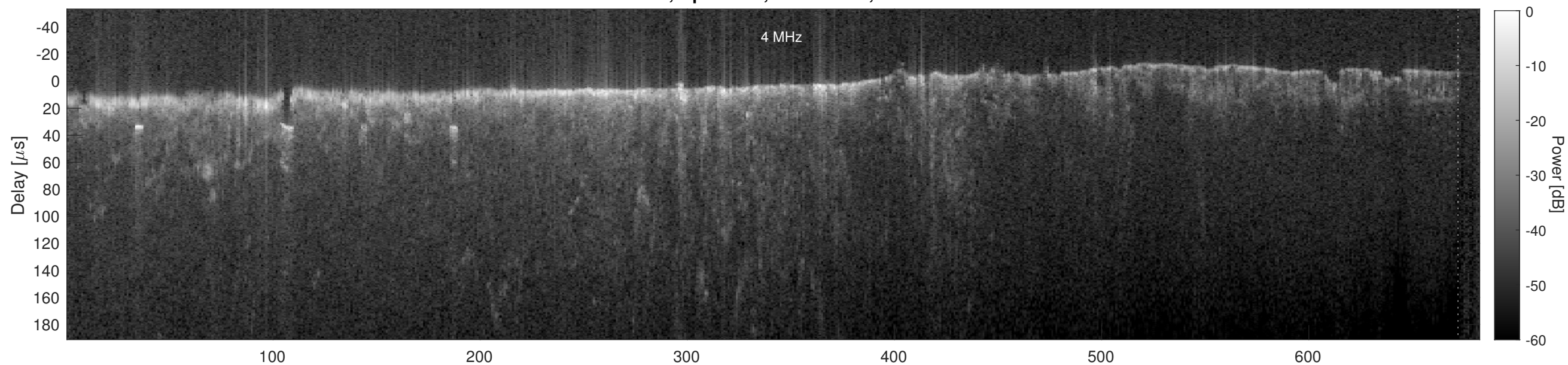
Orbit 4557, Cluttergram
