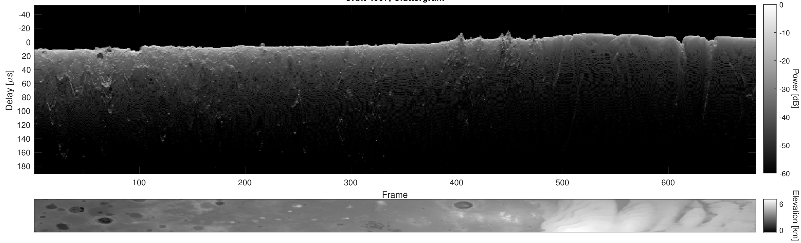
Orbit 4557, Cluttergram
