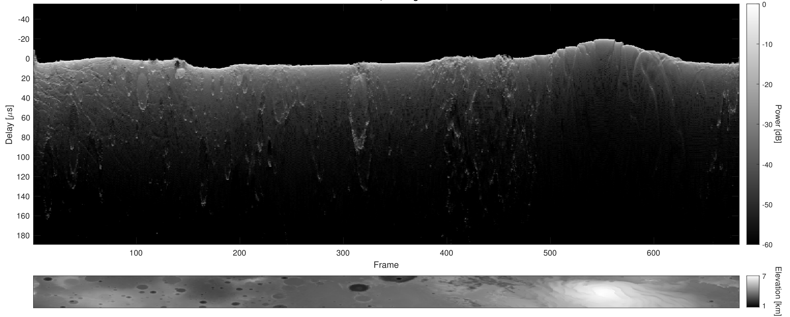
Orbit 4558, Cluttergram
