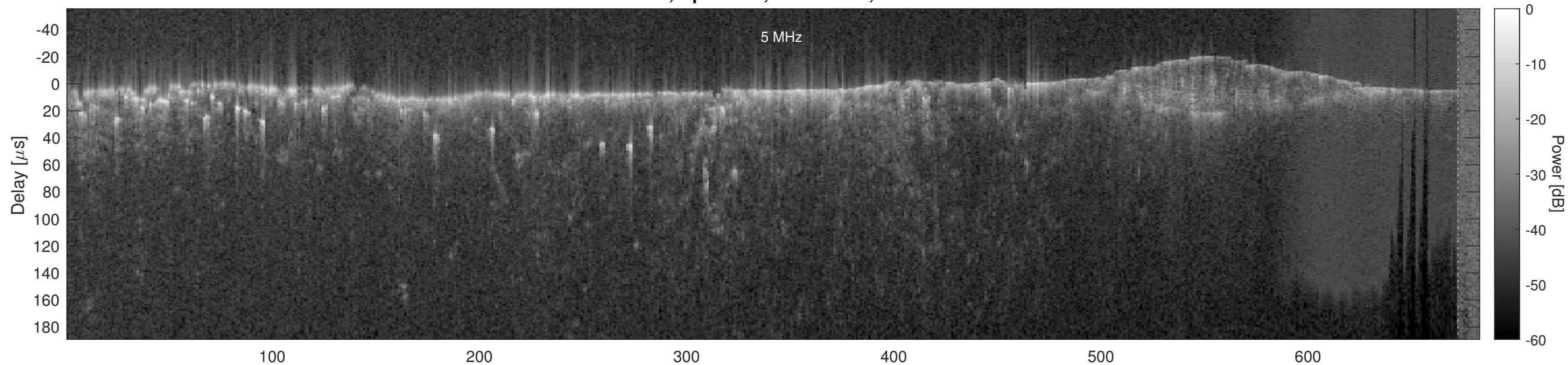
Orbit 4558, Optimized, No Window, Channel 2
