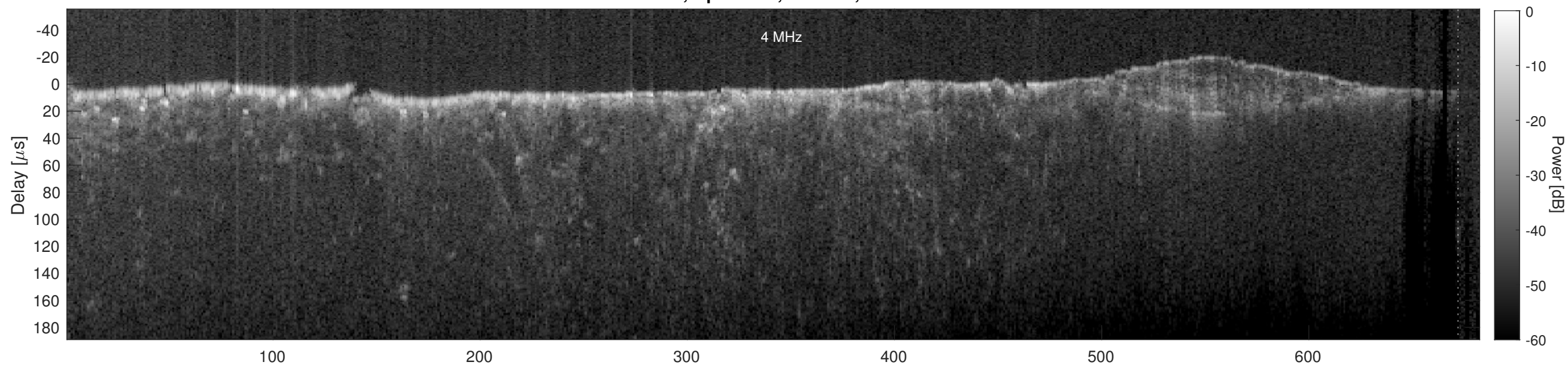
Orbit 4558, Cluttergram
