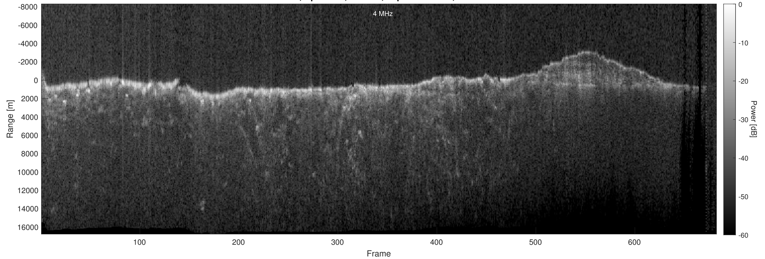
Orbit 4558, Optimized, Window, Depth-Corrected, Channel 2
