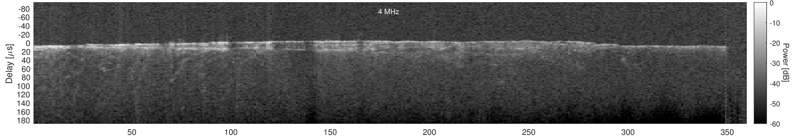
Orbit 4559, Cluttergram
